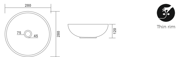
MOON L 280 W 280 H 120mm L 11" W 11" H 5"
