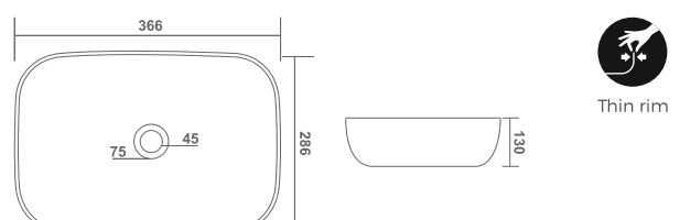
XOLO L 286 W 366 H 130mm L 11" W 15" H 5"
