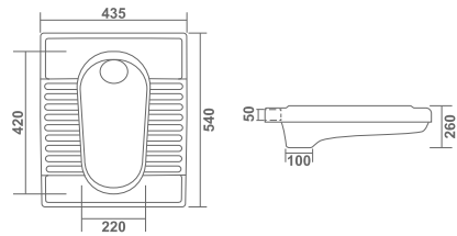
ORISSA PAN 20" L 540 W 435 H 260mm
