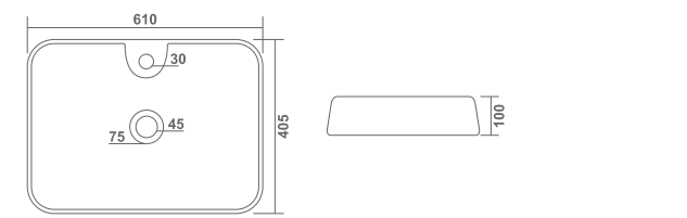
GOLF L 405 W 610 H 100mm L 16" W 24" H 4"
