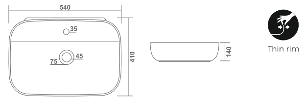
HARMONY L 410 W 540 H 140mm L 16" W 22" H 6"
