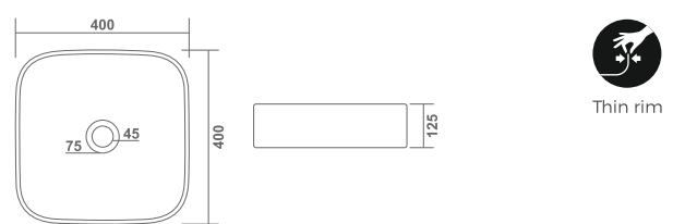
PEARL L 400 W 400 H 125mm L 16" W 16" H 5"
