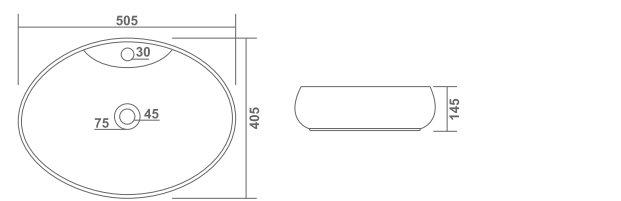
POOL L 405 W 505 H 145mm L 16" W 20" H 6"
