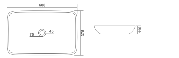
SKING L 375 W 600 H 110mm L 15" W 24" H 4"
