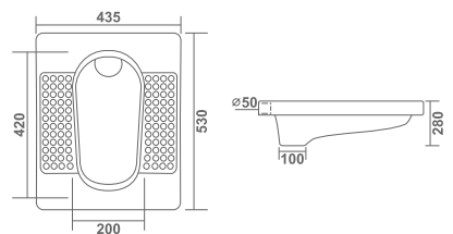
AQUA PAN L 530 W 435 H 280mm
