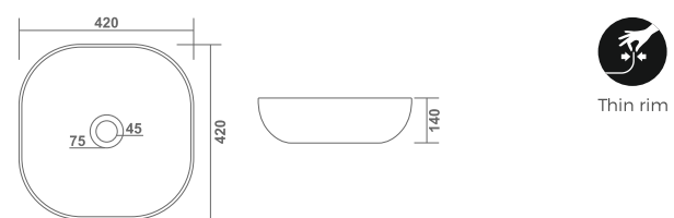
POLIO L 420 W 420 H 140mm L 17" W 17" H 6"
