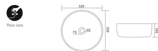
SUN L 320 W 320 H 105mm L 13" W 13" H 4"
